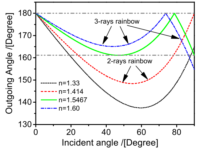
Fig. 2. Incident and scattering angles of primary rainbows of particles with different refractive indices.
