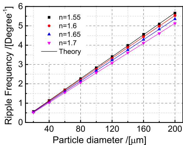
Fig. 4. Angular frequencies of refraction ripples of particles with different high refractive indices and sizes.
