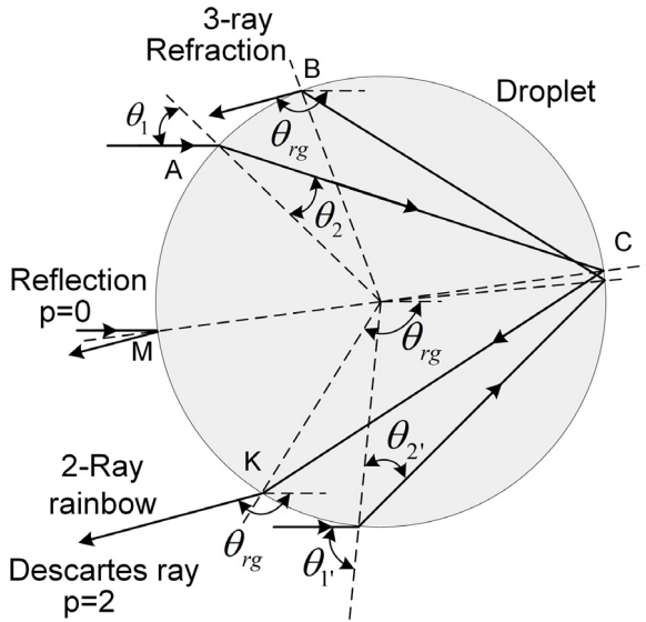
Fig. 1. Ray trajectories of the refraction ( p = 2 ) and reflection ( p = 0 ) light of a particle with high refractive index at the primary rainbow with geometrical optics.
