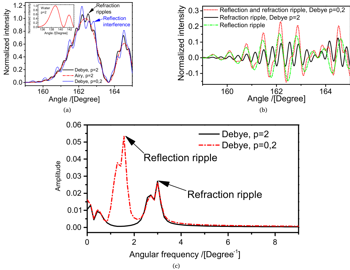
Fig. 3. Rainbow light behaviors of a particle with n = 1.55 and d = 100 \mu\text{m} , under 532 nm laser illumination. (a) Primary rainbow and its comparison with that of Airy theory and Debye series ( p = 0, 2 ). (b) Refraction ripples of Primary rainbow and its comparison with reflection ripples. (c) Angular frequencies of rainbow ripples.
